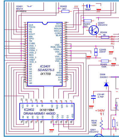
Fig. 15: IC2401-IC2402 configuration.
