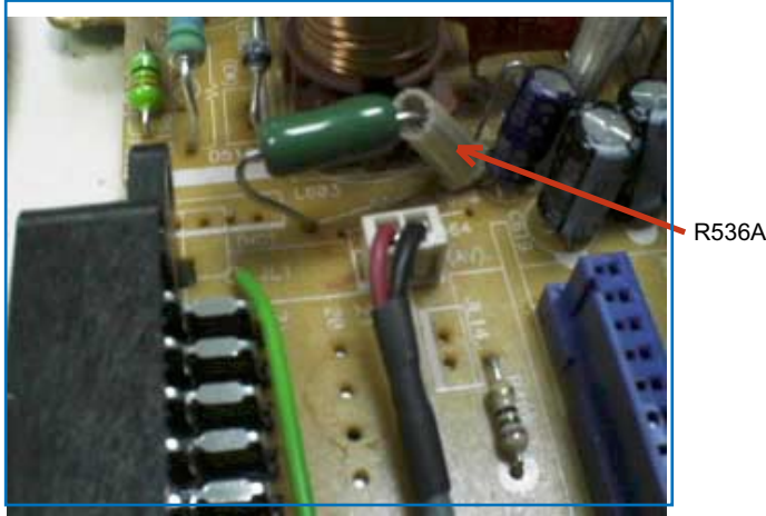
Fig. 14: How to assemble R536A (Vinyl tube for R536).
